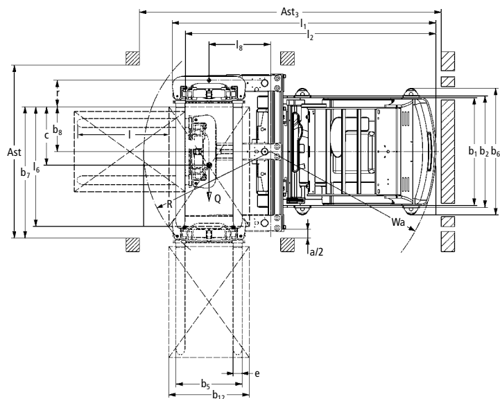
Standard Values For Working Aisle Widths Pallet Size Stacking-in Depth Clear Aisle Width (AST)* Transfer Aisle (AST 3 ) Theoretical Transfer Aisle (AST 3 ) Practical*** With Rail Guidance in mm in mm in mm in mm in mm 48 x 48 1,219 x 1,219 48.0 1,219 70 1,778 147.6 3,749 +20.0 +508 48 x 40 1,219 x 1,016 48.0 1,219 70** 1,778 131.3 3,335 +20.0 +508 With Wire Guidance in mm in mm in mm in mm in mm 48 x 48 1,219 x 1,219 48.0 1,219 72 1,829 147.6 3,749 +40.0 +508 48 x 40 1,219 x 1,016 48.0 1,219 72 1,829 131.3 3,335 +40.0 +508 * Up to h 3 = 157.5 inches; +0.8 inches for h 3 > 157.5-236.2; +2.8 inches for h 3 > 236.2 inches. ** Lower values possible if lower rail guide rollers are used. *** The practical transfer aisle width is a reference value.
